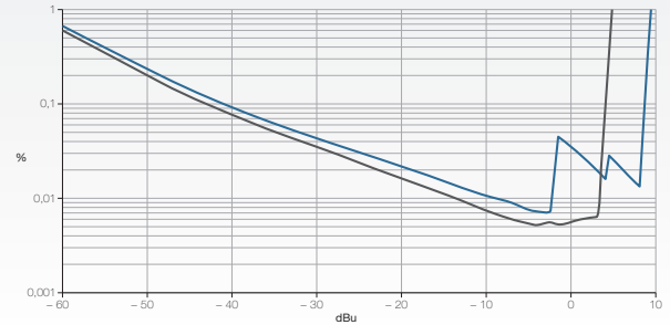
8.3 THD @ 1 kHz vs. input level @ 2 Ω load 32 dB amplifier gain (Measurement of a typical performance of a iD4 & iD7 )
