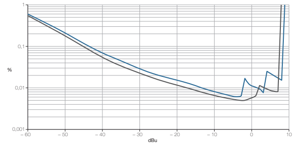
8.4 THD @ 1 kHz vs. input level @ 4 Ω load 32 dB amplifier gain (Measurement of a typical performance of a iD4 & iD7 )
