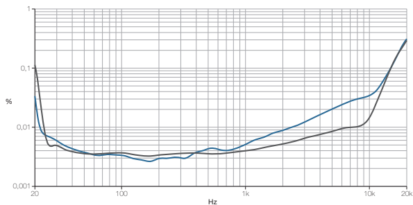
8.6 THD vs. frequency, 120 W output power @ 4 Ω load (Measurement of a typical performance of a iD4 & iD7 )
