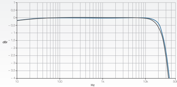
8.1 Gain vs. frequency, 120 W output power @ 2 Ω load (Measurement of a typical performance of a iD4 & iD7 )
