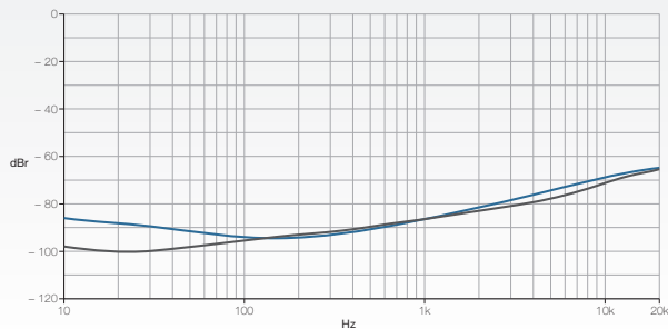
8.7 Channel separation vs. frequency @ 120 W / 4 Ω (Measurement of a typical performance of a iD4 & iD7 )
