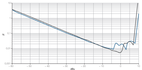
8.8 DIM100 vs. input level @ 4 Ω load 32 dB amplifier gain (Measurement of a typical performance of a iD4 & iD7 )
