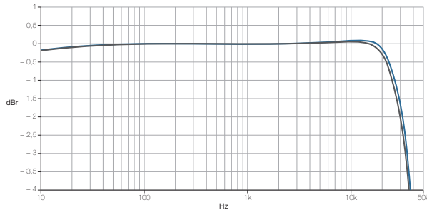
8.2 Gain vs. frequency, 120 W output power @ 4 Ω load (Measurement of a typical performance of a iD4 & iD7 )
