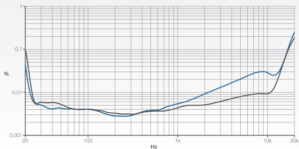
8.5 THD vs. frequency, 120 W output power @ 2 Ω load (Measurement of a typical performance of a iD4 & iD7 )
